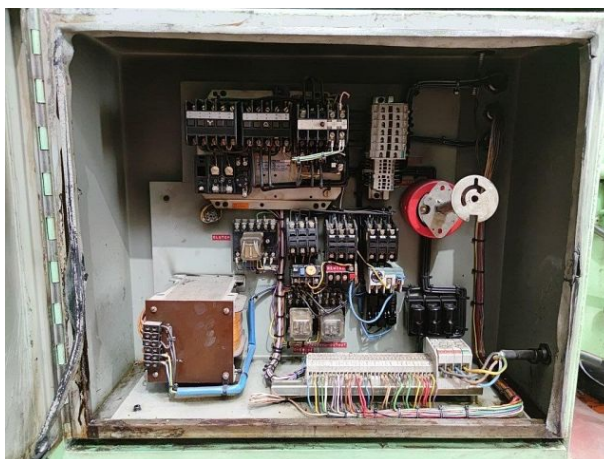
Electrical Cabinet
