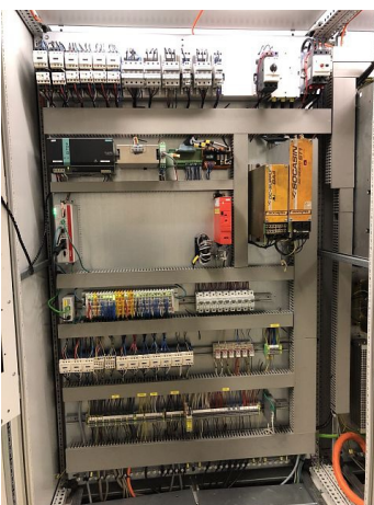
Electrical Cabinet Inside
